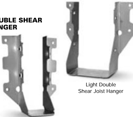
Light Shear Joist Hanger
