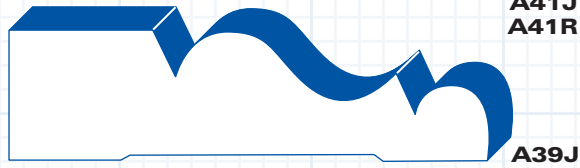
A40J Paint Grade Fluted Pilaster 1 1/16" x 5 1/2"
