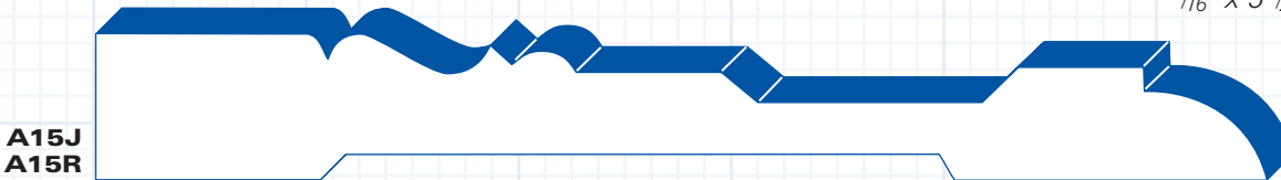
A16R Redwood/ Red Cedar Bell Casing 1 1/16" x 5 1/2"
