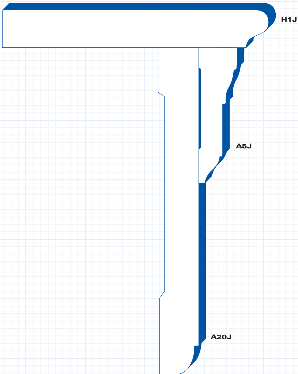
Window Sill
